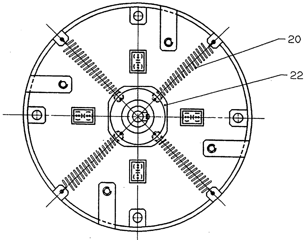
SECTION C-C - FIG 5
